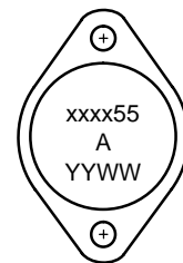
TO-204AA (TO-3) CASE 1-07
